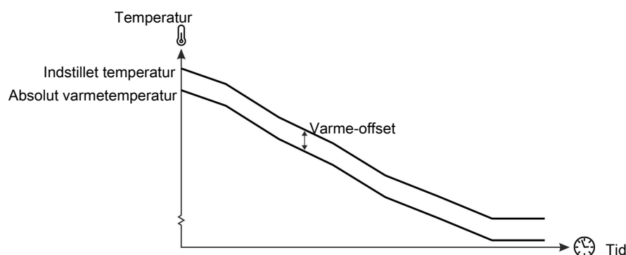
Figur 36: Indstillet varmer-offset
