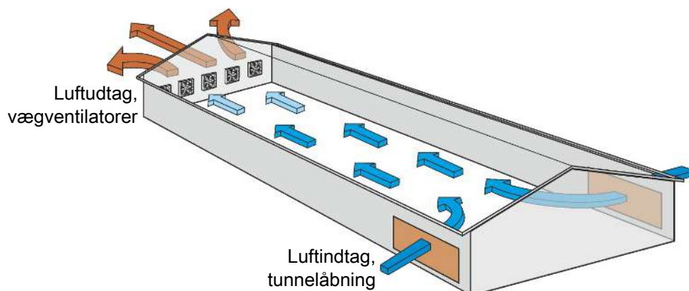
Figur 1: Princip for tunnelventilation
